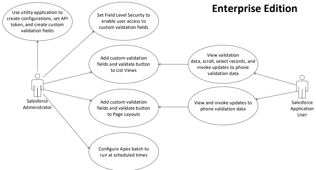
Figure 1: Phone Validation Use Cases
